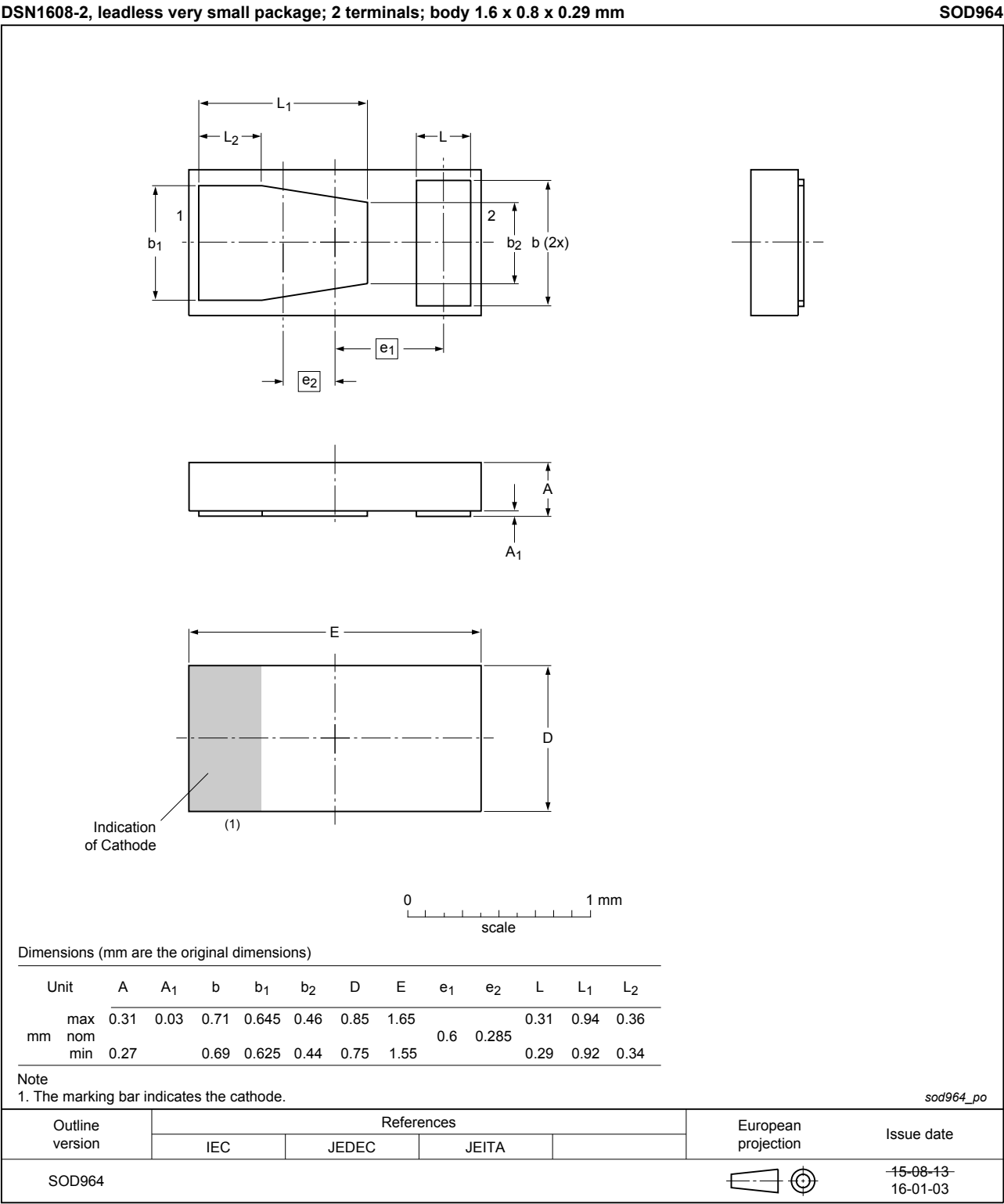
Fig. 14. Package outline DSN1608-2 (SOD964)
