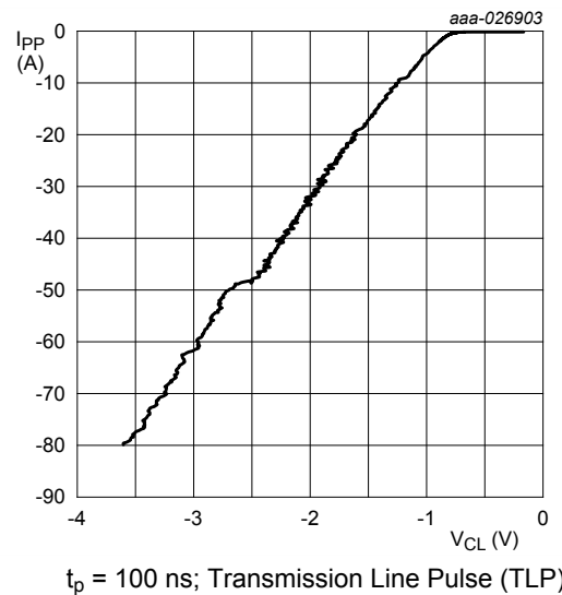
Fig. 11. Dynamic resistance with negative clamping voltage; typical values
