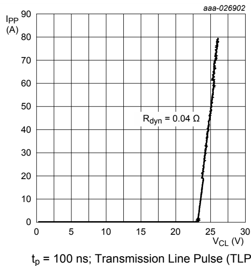
Fig. 10. Dynamic resistance with positive clamping voltage; typical values
