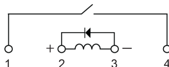
Schematic View
