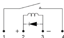
Schematic View
