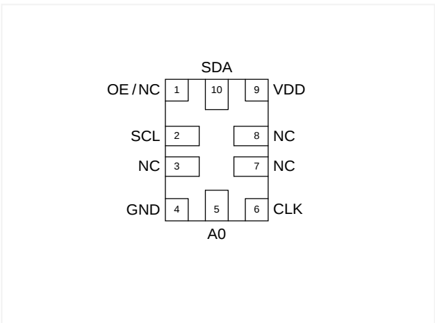
Figure 28. Top-View - DCTCXO
