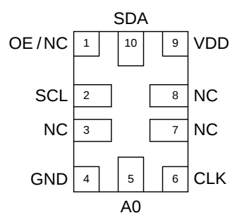
Figure 5. DCTCXO
