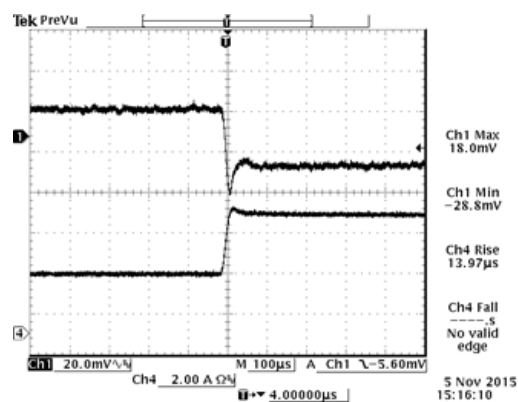
Figure 12. 50%-100% Load Transients at V_{in}=12\text{V} , V_{out}=0.6\text{V} at T_a=25^\circ\text{C}
