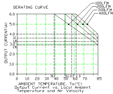
Figure 7. V_{out} = 5.5V
