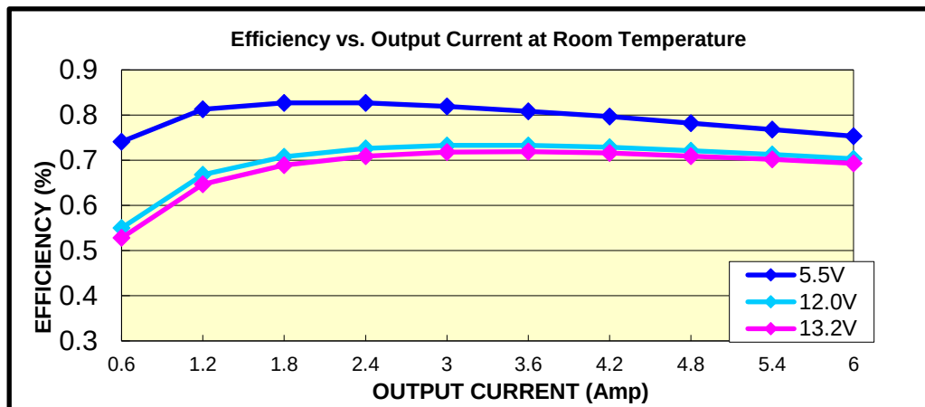
Figure 1. V_{out} = 0.6 V
