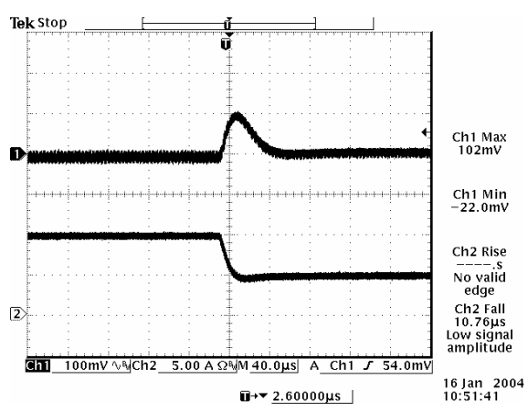
Transients 100% to 50% load 3.3 Vdc output
