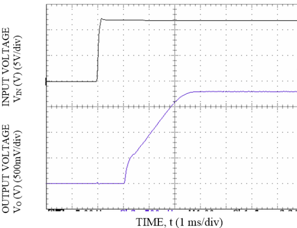
Figure 26. Start-up Using Input Voltage ( V_{IN} = 12V , I_o = I_{o,max} ), V_o = 1.8V
