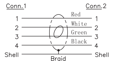
Pin Assignment
