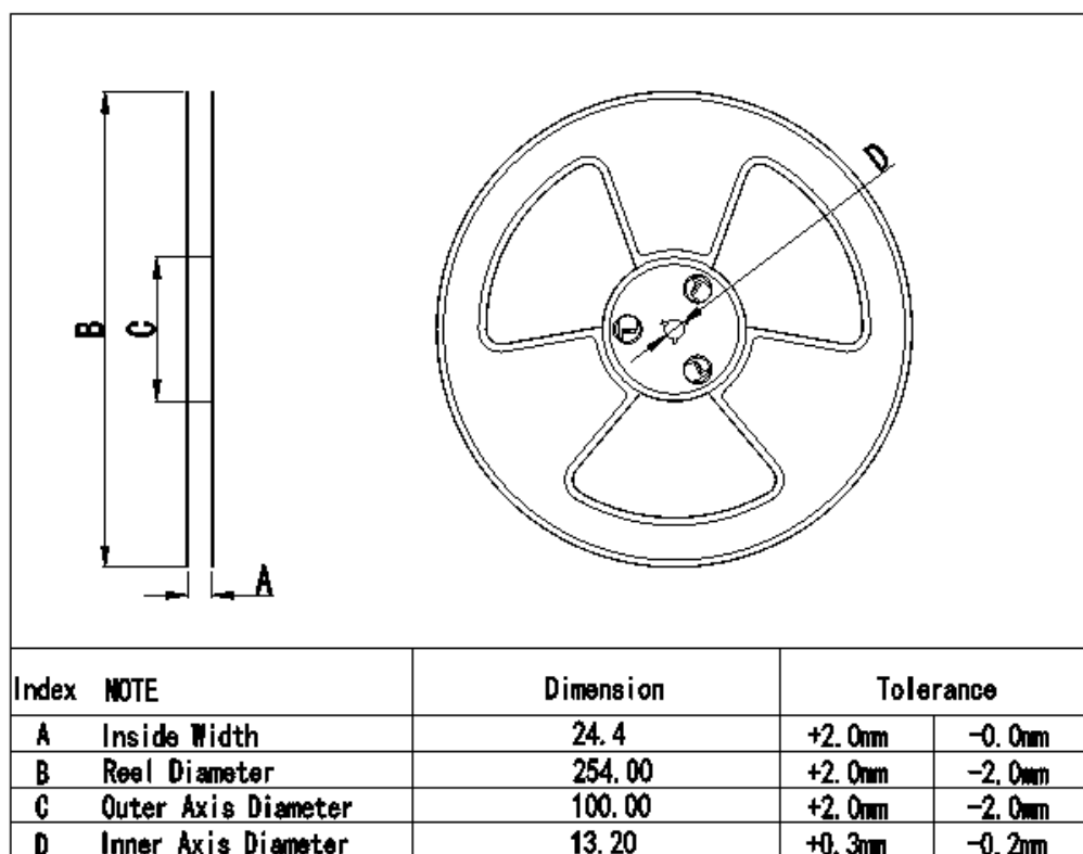
Figure 22. Reel Dimensions
