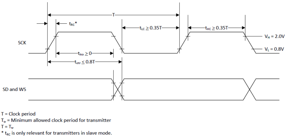
Figure 18. I 2 S Transmitter Timing
