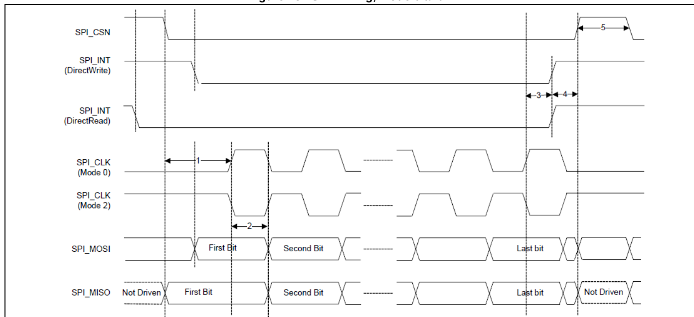
Figure 15. SPI Timing, Mode 0 and 2
