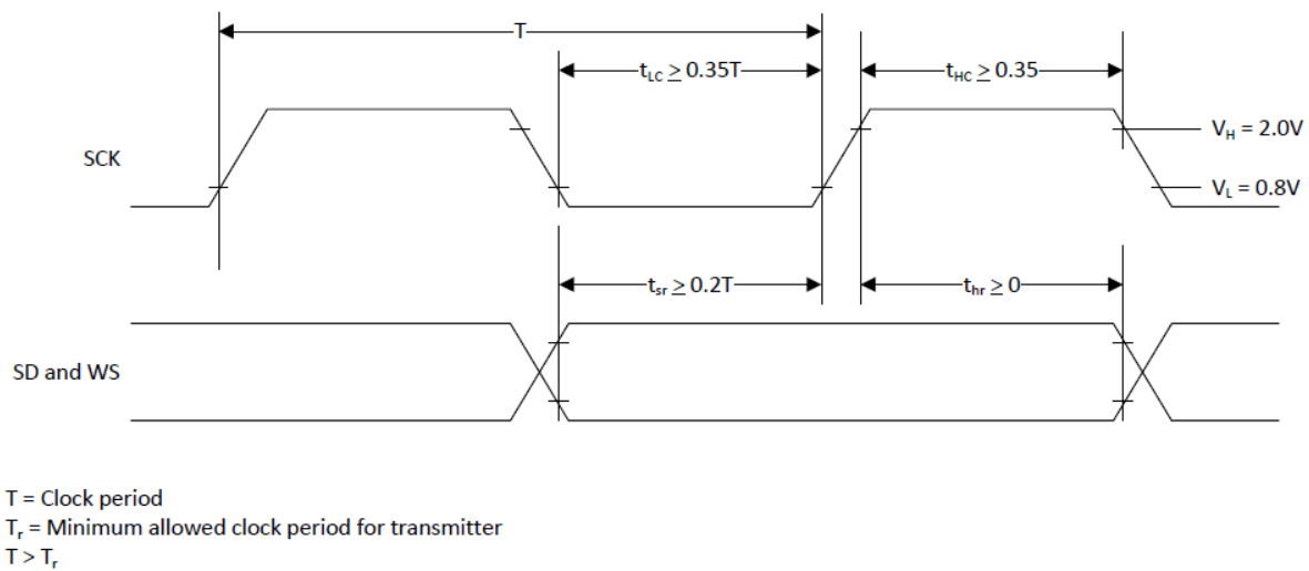
Figure 19. I 2 S Receiver Timing
