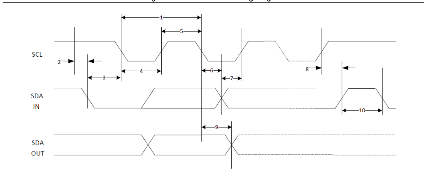
Figure 17. I 2 C Interface Timing Diagram
