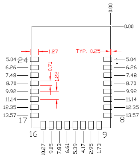
Figure 6. CYBT-343026-01 Host Layout (Relative to Origin)
