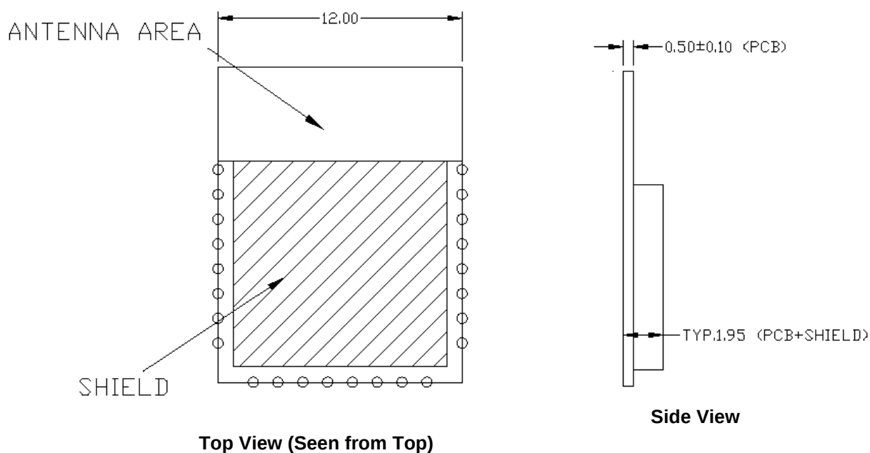
Figure 2. Module Mechanical Drawing [2, 3]
