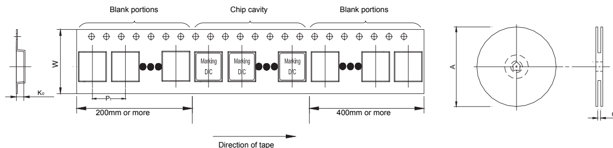
SURFACE MOUNTING TYPE, REEL/TAPE LIST
