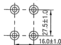
Mounting Holes
