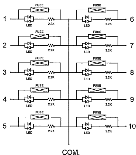
Circuit Diagram
