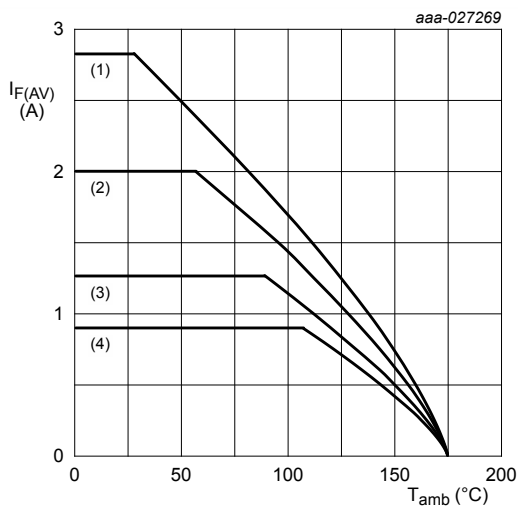
FR4 PCB, mounting pad for cathode 1\text{ cm}^2 T_j = 175\text{ }^{\circ}\text{C} (1) \delta = 1 ; DC (2) \delta = 0.5 ; f = 20\text{ kHz} (3) \delta = 0.2 ; f = 20\text{ kHz} (4) \delta = 0.1 ; f = 20\text{ kHz}
