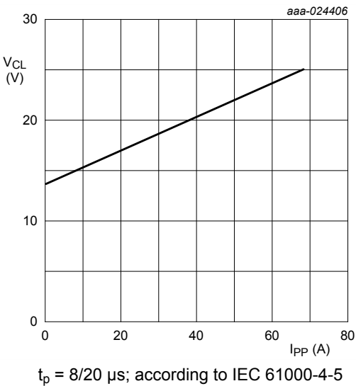
Fig. 10. Positive clamping voltage (8/20 μs pulse); typical values
