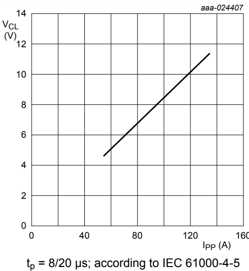
Fig. 11. Negative clamping voltage (8/20 μs pulse); typical values
