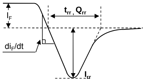
Fig.25 Diode Reverse Recovery Waveform
