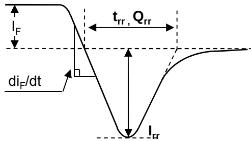
Fig.25 Diode Reverse Recovery Waveform
