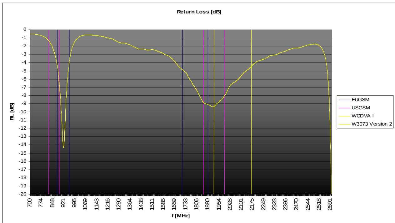
Version 2: Typical Return Loss S11
