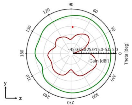
Phi = 90
