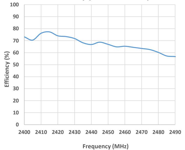
Efficiency (2400 – 2490 MHz)
