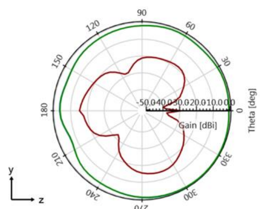
Phi = 90
