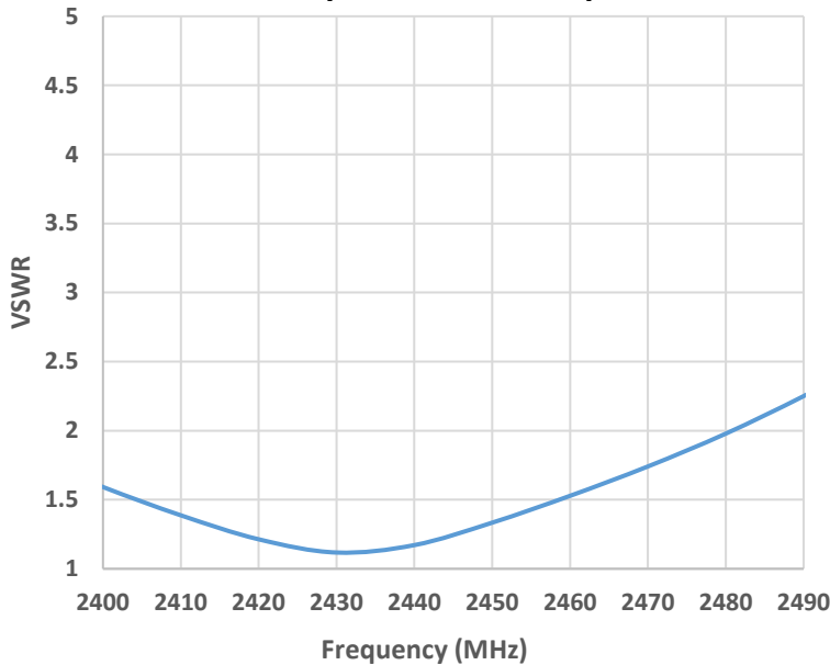
VSWR (2400 – 2490 MHz)
