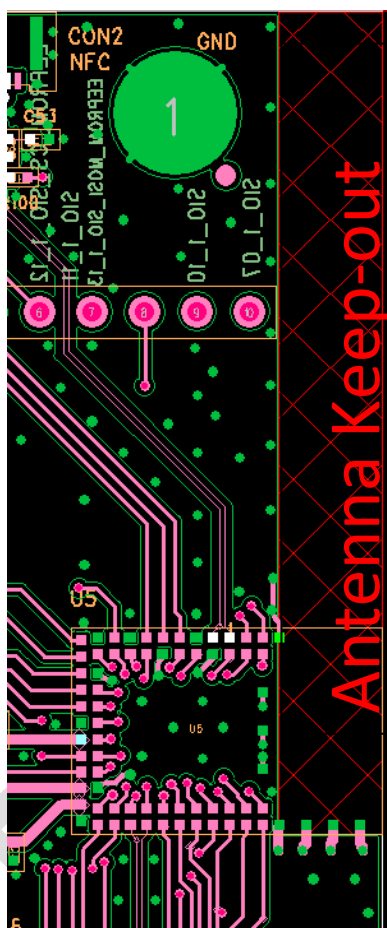
Figure 8: PCB trace Antenna keep-out area (shown in red), corner of the BL654 development board for the 451-00001 module.
