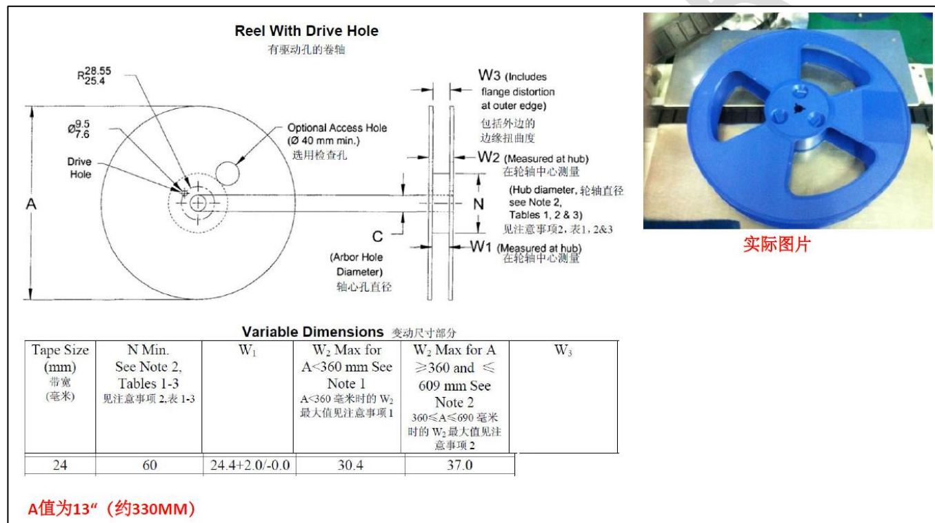
Figure 11: Reel specifications
