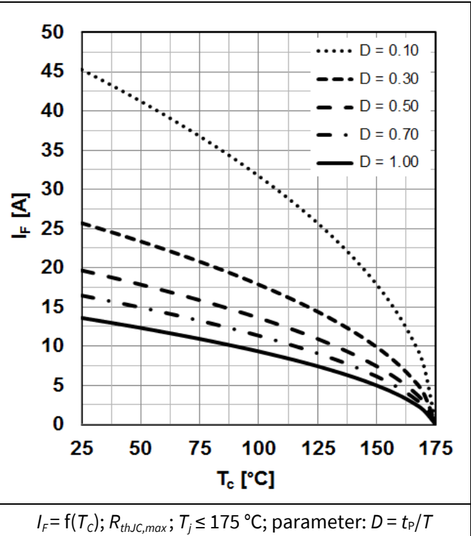
Figure 2 Max. forward current
