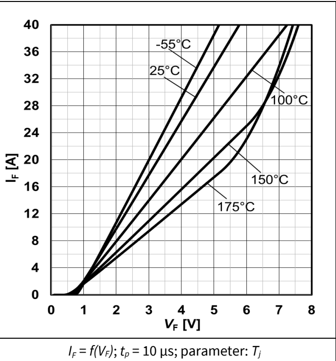
Figure 4 Typ. forward characteristics in surge current
