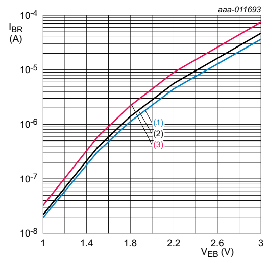
V_{CE} = 3 V. (1) T_{amb} = -40\text{ }^{\circ}\text{C} (2) T_{amb} = +25\text{ }^{\circ}\text{C} (3) T_{amb} = +125\text{ }^{\circ}\text{C}
