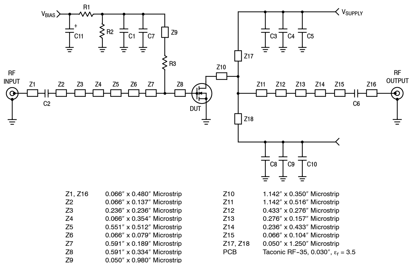
Figure 23. MRF6S20010NR1 Test Circuit Schematic — 1805-1880 MHz
