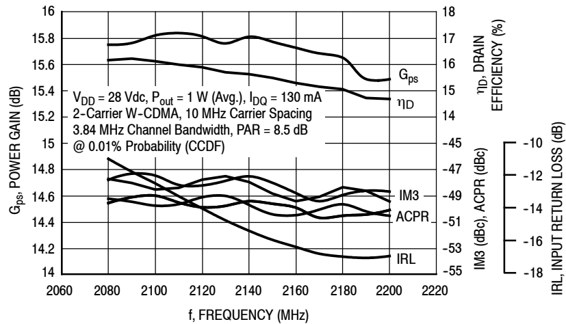
Figure 13. 2-Carrier W-CDMA Broadband Performance @ P_{out} = 1 \text{ Watt Avg.}
