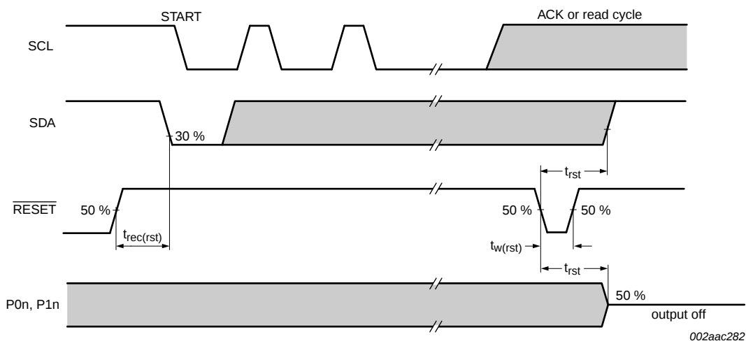
Fig 25. Reset timing
