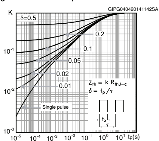
Figure 3. Thermal impedance for TO-3PF
