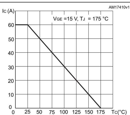
Figure 5. Collector current vs. case temperature for TO-3PF
