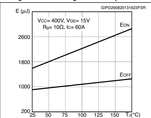
Figure 13. Switching loss vs temperature
