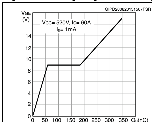
Figure 12. Gate charge vs. gate-emitter voltage
