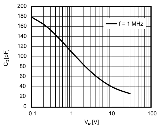
Fig. 2 - Typical Diode Capacitance vs. Reverse Voltage
