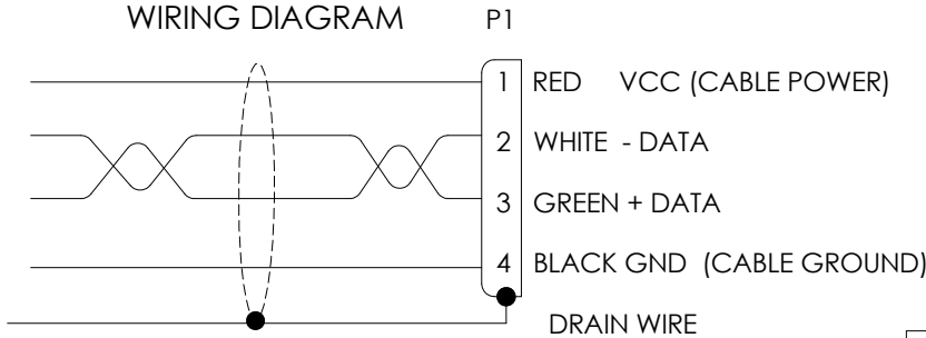
WIRING DIAGRAM
