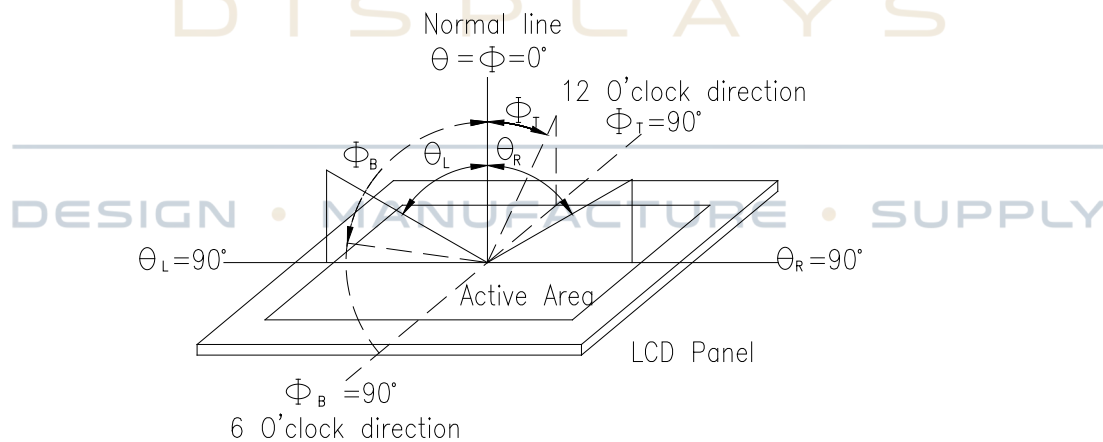
Fig. 9.1. Definition of viewing angle
