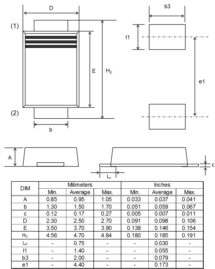
SOD-128, (PMD™)
