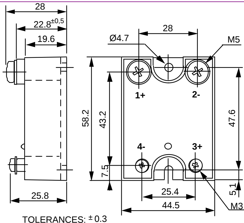
DIMENSIONS (mm)
