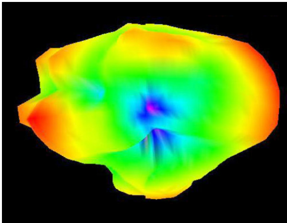
2690 MHz
