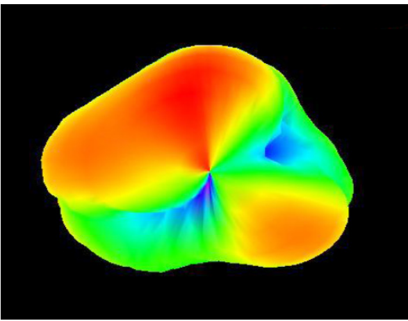
868 MHz
