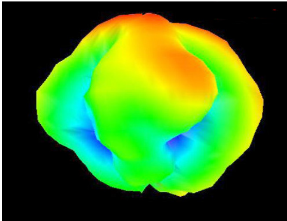
1990 MHz
