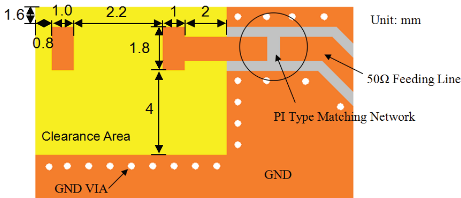
Layout Dimensions
