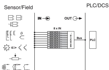
Block diagram
