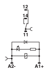
Circuit diagram
