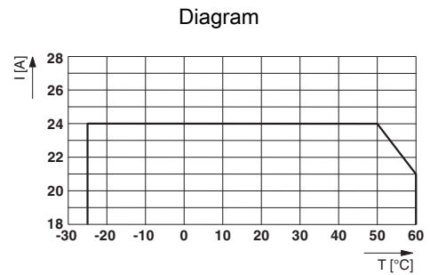
Total current input
