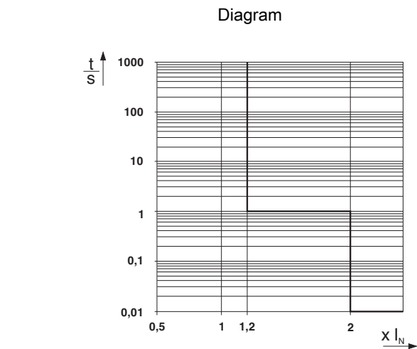
Trigger characteristic in the DC range
