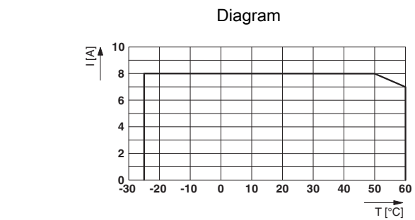
Channel current output
