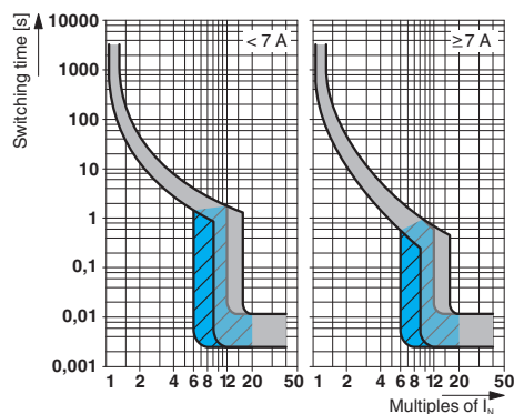
Trigger characteristic
