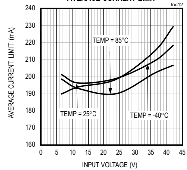
AVERAGE CURRENT LIMIT
