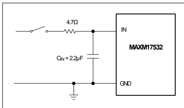
Figure 4. Circuit for Transient Protection
