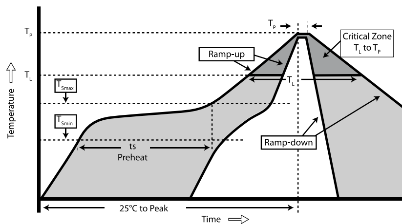
Figure 15. Soldering profiles
