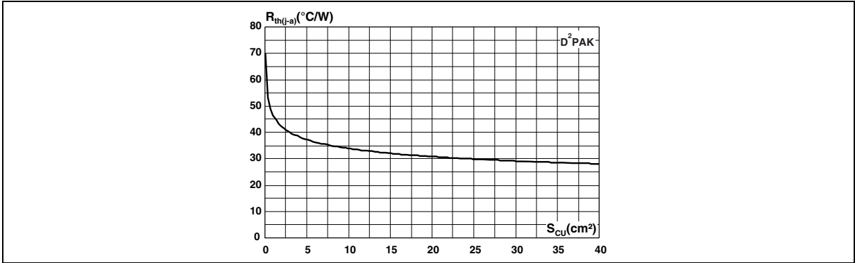
Figure 11. Thermal resistance junction to ambient vs. copper surface under tab (D 2 PAK, printed circuit board FR4, copper thickness: 35 µm)
