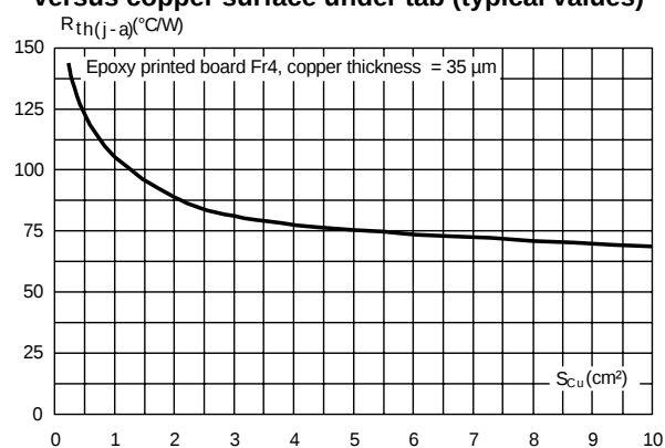
Figure 7: Thermal resistance junction to ambient versus copper surface under tab (typical values)
