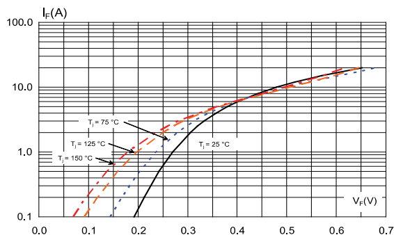
Figure 5: Forward voltage drop versus forward current (typical values, per diode)
