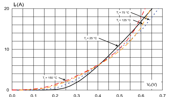
Figure 6: Forward voltage drop versus forward current (typical values, per diode)
