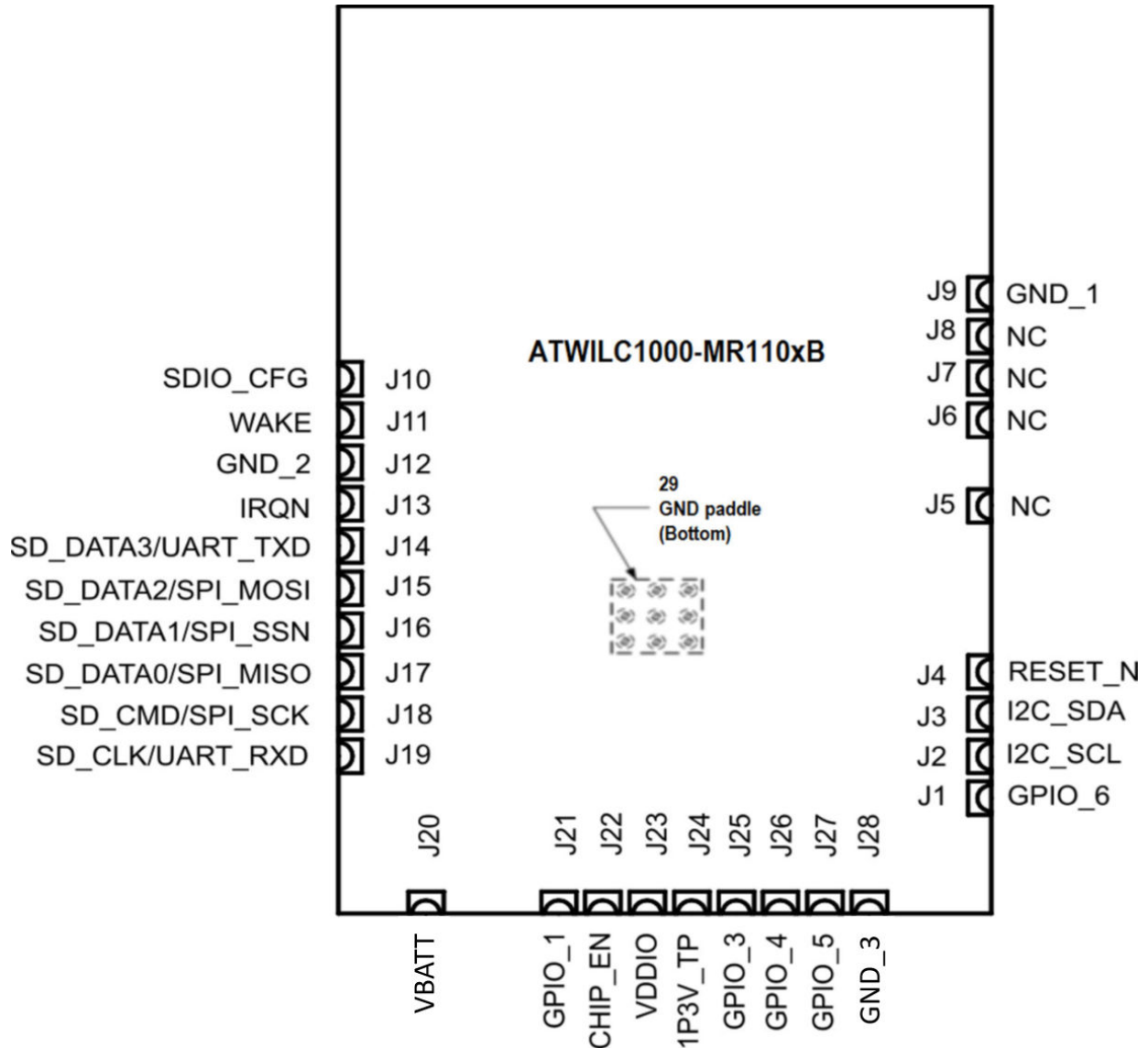
Figure 3-1. Pin Assignment
