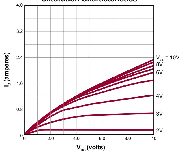
Saturation Characteristics
