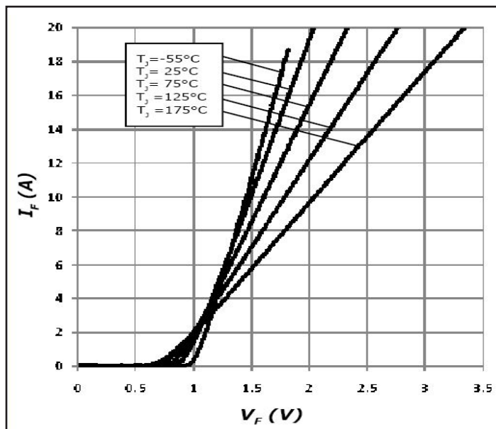
Figure 1. Forward Characteristics
