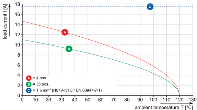
B2CF 3.50/..180 - S2C-SMT 3.50/..90
