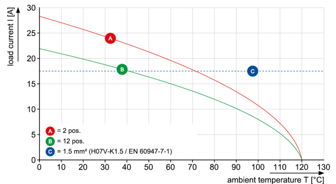
LSF-SMD 3.5/..180
