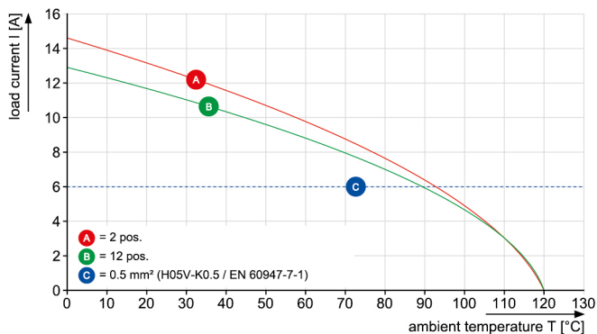
LSF-SMD 3.5/..180
